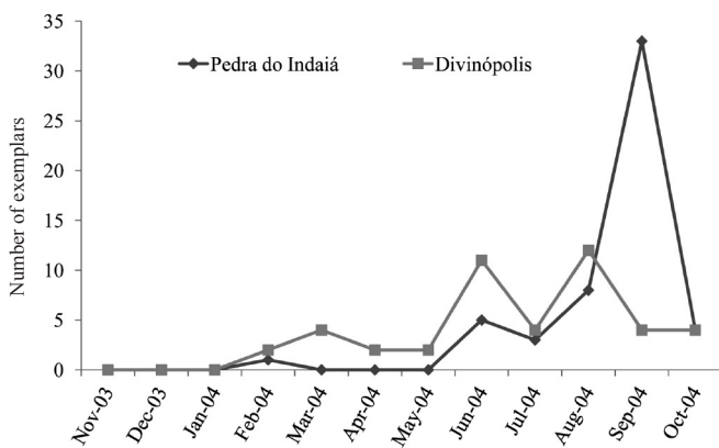
Figure 1. Fluctuation in the population of Nusalala tessellata Gerstaecker (Neuroptera, Hemerobiidae) collected in areas of Brazilian savannah and gallery forest in Divinópolis and Pedra do Indaiá, Minas Gerais State, Brazil, respectively. Period of collection between November 2003 and October 2004.
